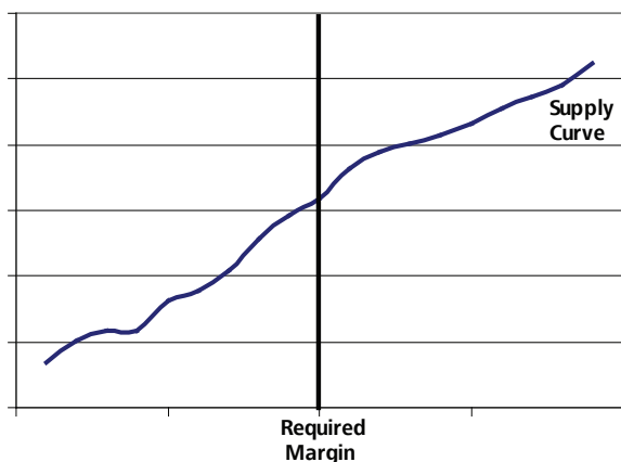
Figure 1 Auction Mechanism with a Fixed Quantity as the Demand
