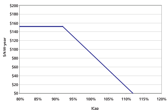
Figure 2 Auction Mechanism with a Demand that Depends on Price
