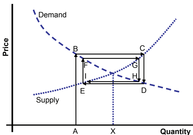
Figure 1: The Cobweb Theory
